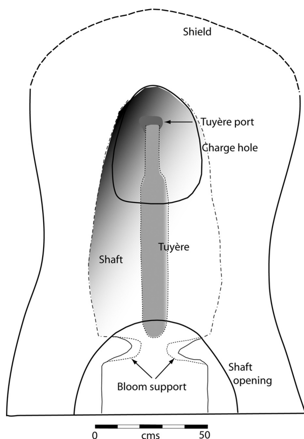
Figure 8: Diagrammatic frontal reconstruction of the Mazavā 1 furnace, drawn from photographs and field measurements. The daub bloom support is horseshoe-shaped and open to the front. Tuyère length is estimated at 103cm.
