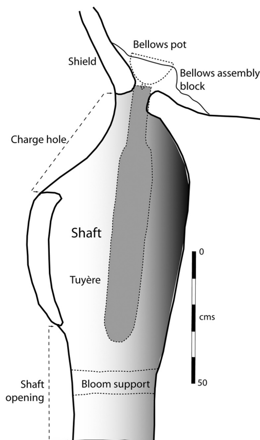
Figure 9: Diagrammatic cross-sectional reconstruction of the Guili 1 furnace, drawn from photographs and field measurements. The partially-reconstructed lines of the daub bloom support are indicated. Tuyère length is estimated at 98cm.
