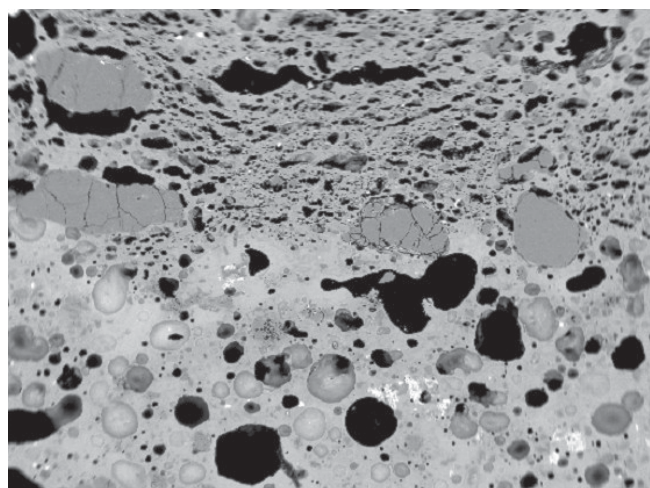
Figure 9: Backscattered electron image of the interface between the ceramic fabric of a type C crucible (top) and the external ceramic wrap (bottom). Note the increased number of round voids and more vitrified quality of the less-refractory wrap, in contrast to the fine pores of the quartz-tempered body. Width of image c3mm.
