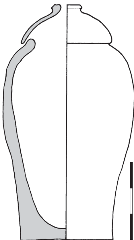
Figure 12: Reconstruction of the lidded cementation crucibles. Type A vessels with type B lids. Scale bar 150mm. (Drawing J Beutmann).
