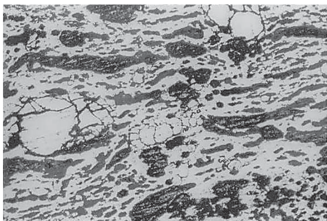
Figure 3: Backscattered electron image of the ceramic fabric of a type A crucible, with fine to coarse voids (dark) developing within a dense matrix. Note the abundance of (mid-grey) quartz grains. Width of image c3mm.
