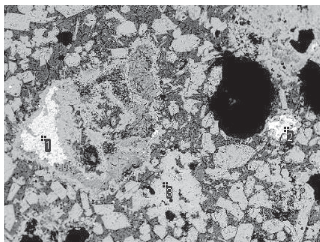
Figure 5: Backscattered electron image of slag layer within a type A crucible. Bright area 1 is metallic zinc, area 2 is a copper droplet, white crystals 3 are richer in zinc oxide, within a matrix containing more FeO and \text{Al}_2\text{O}_3 . Width of image c600 \mu\text{m} .
