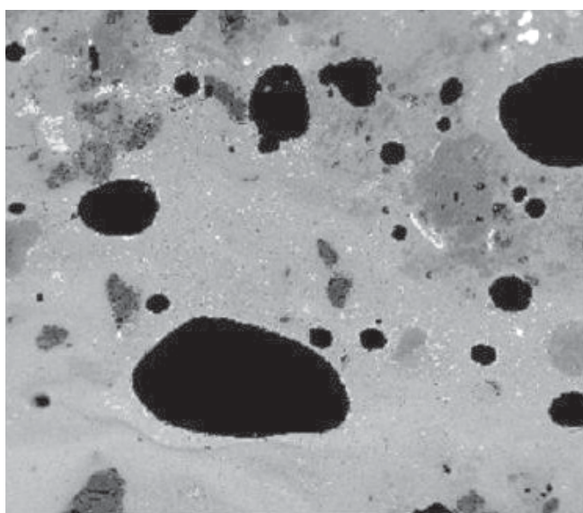
Figure 4: Backscattered electron image of the external ceramic wrap of a type A crucible, highly vitrified with a few quartz grains in the matrix. The bright areas (top and top left) are titanium minerals and the white spots (top right) are droplets of copper with Zn, Fe and Ni. Width of image c3mm.
