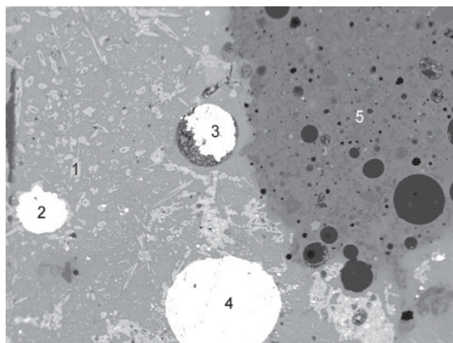
Figure 11: Backscattered electron image of the slag layer within a type C crucible. (1) zinc-rich crystals within the matrix, (2-4) circular droplets of copper with Zn, Ni, As and Fe, (5) large siliceous inclusion. Width of image c3mm.
