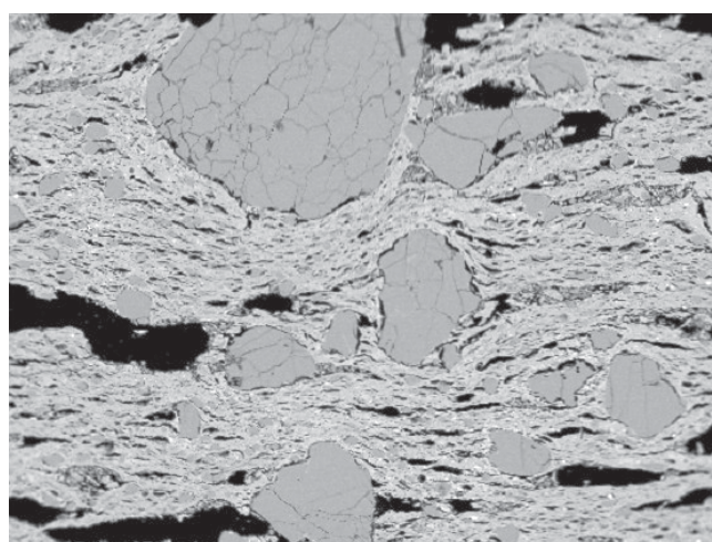
Figure 7: Backscattered electron image of ceramic fabric of a type B crucible, showing abundant unreacted quartz grains of various sizes surrounded by expansion voids, and elongated cracks parallel to the surface of the sherd. The matrix is not very vitrified. Width of image c30mm.
